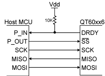
Figure 3-1 SPI Connections
