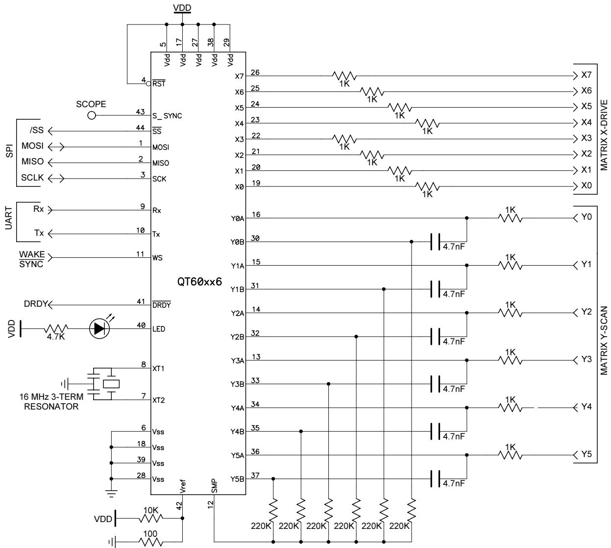
Figure 2.1 Wiring Diagram
