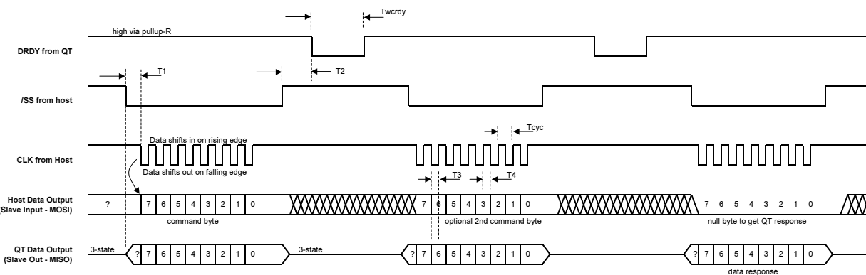
Figure 3-2 SPI Slave-Only Mode Timing
