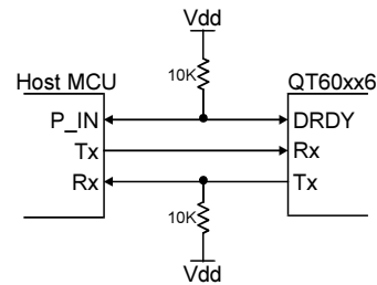
Figure 3-3 UART Connections
