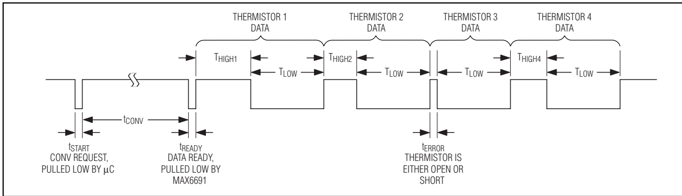
Figure 1. Timing Diagram
