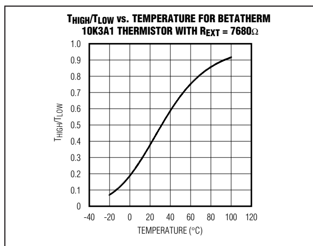
Figure 4. T_{HIGH}/T_{LOW} vs. Temperature, R_{EXT} = 7680\Omega
