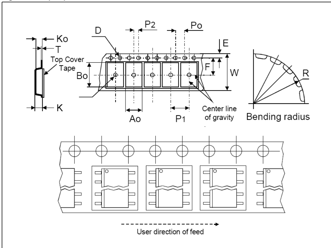
Figure 14. Tape Specification
