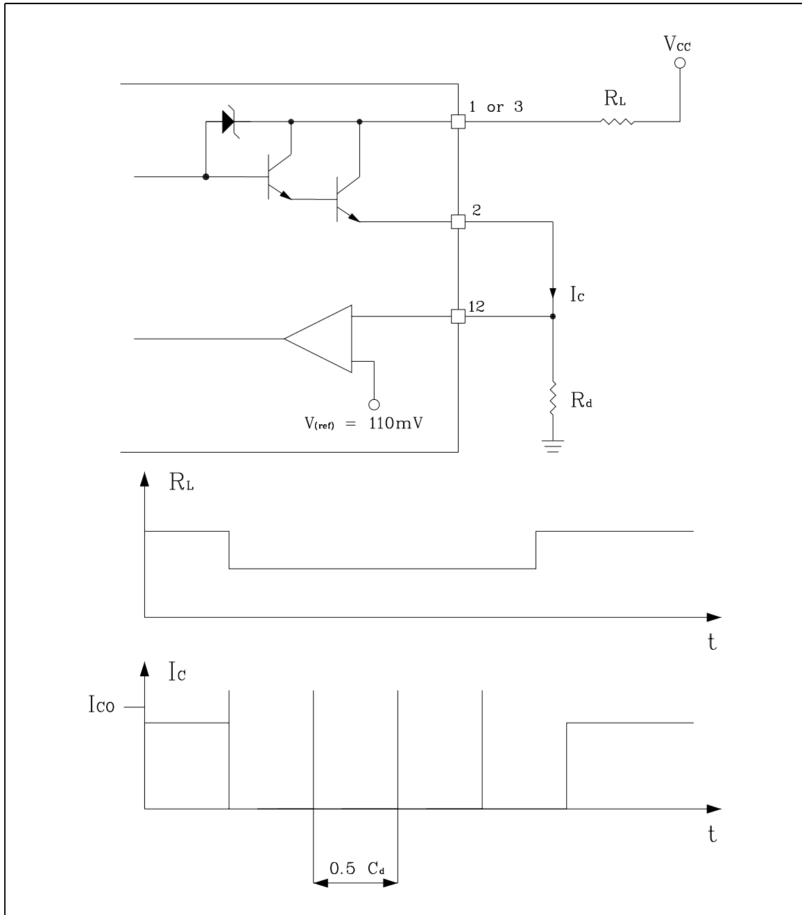
Figure 2. Switching Operation
