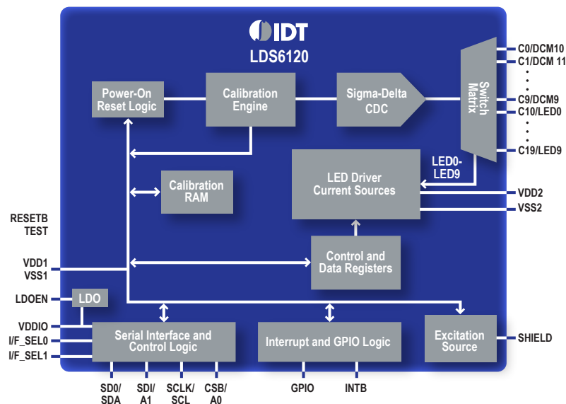
Figure 1. LDS6120 block diagram
