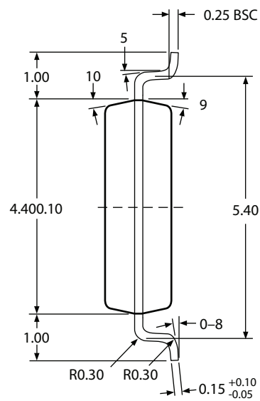
End View
