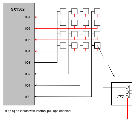
Figure 14 – 4x4 keypad connection to SX1505
