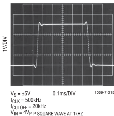
Transient Response
