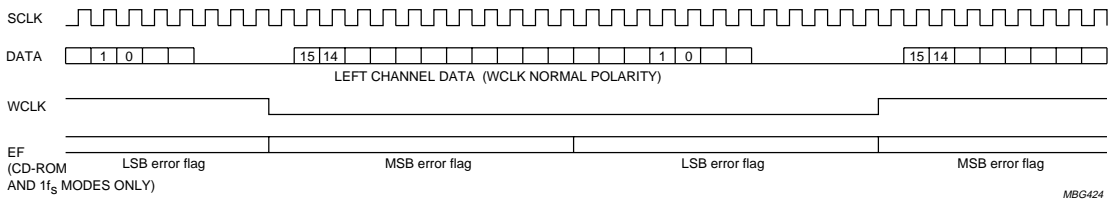
Fig.14 Philips I 2 S-bus data format (16-bit word length).
