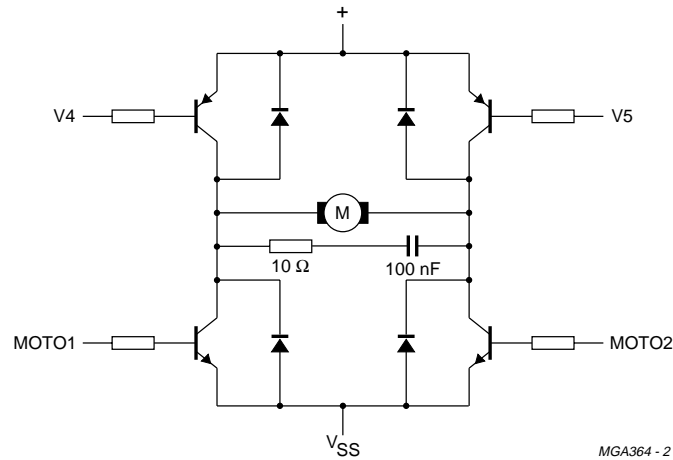
Fig.19 Motor 4-line PWM mode application diagram.
