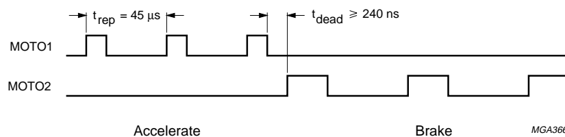
Fig.16 2-line PWM mode timing.
