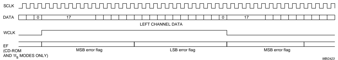
Fig.15 EIAJ data format (18-bit word length).
