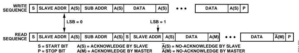
Figure 39. Read and Write Sequence
