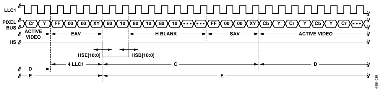
Figure 19. HS Timing
