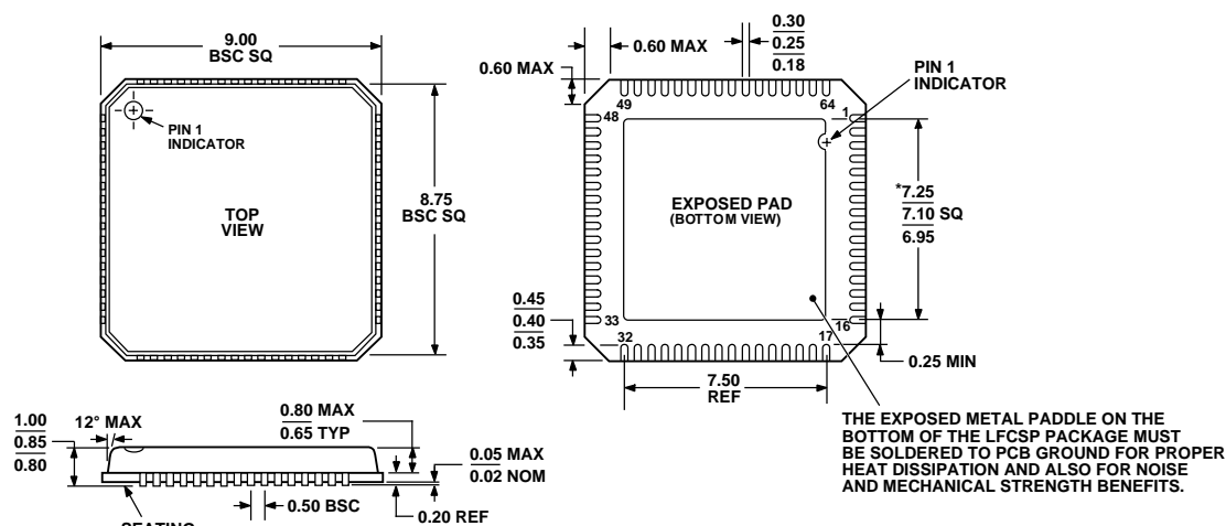
Figure 46. 64-Lead Lead Frame Chip Scale Package [LFCSP_VQ] 9 × 9 mm Body, Very Thin Quad (CP-64-3) Dimensions shown in millimeters
