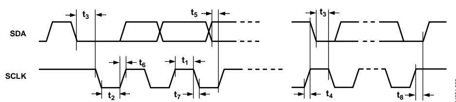
Figure 2. I²C Timing
