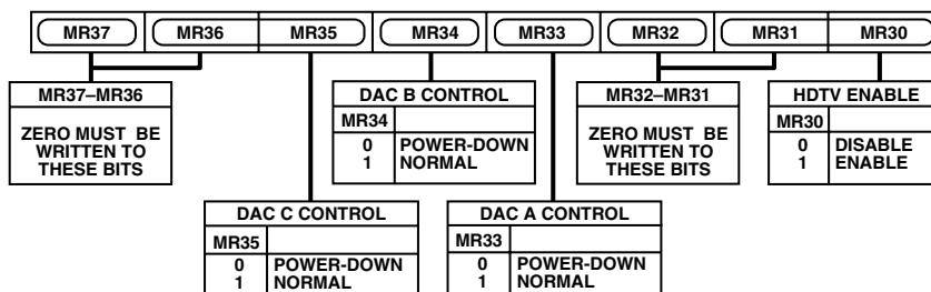
Figure 54. Mode Register 3
