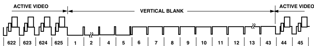
Figure 68. ITU-R.BT1358 (625p)
