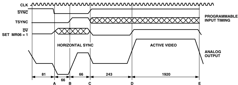
Figure 48. Async Timing Mode—Programming Input Control Signals for SMPTE295M Compatibility
