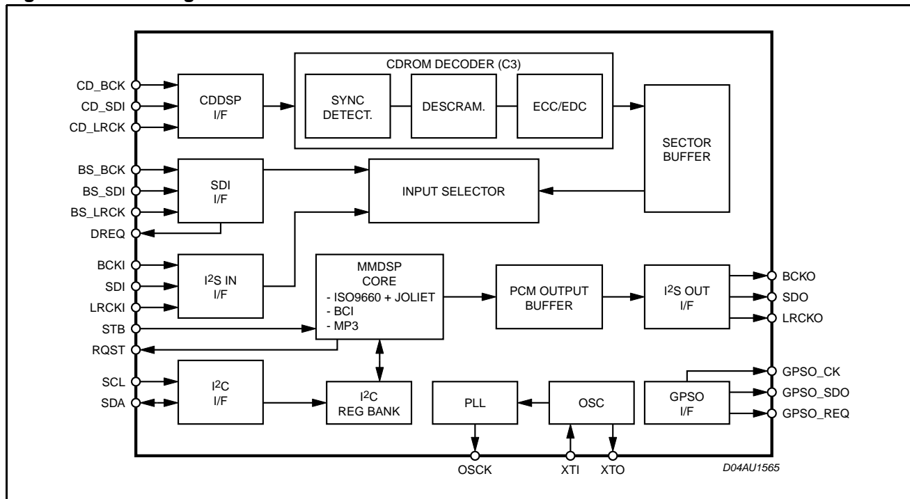
Figure 3. Block Diagram
