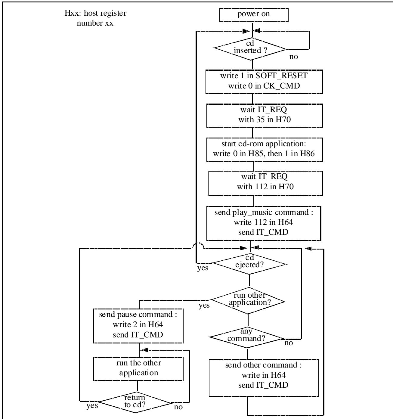
Figure 7. Block diagram for running the CD application.
