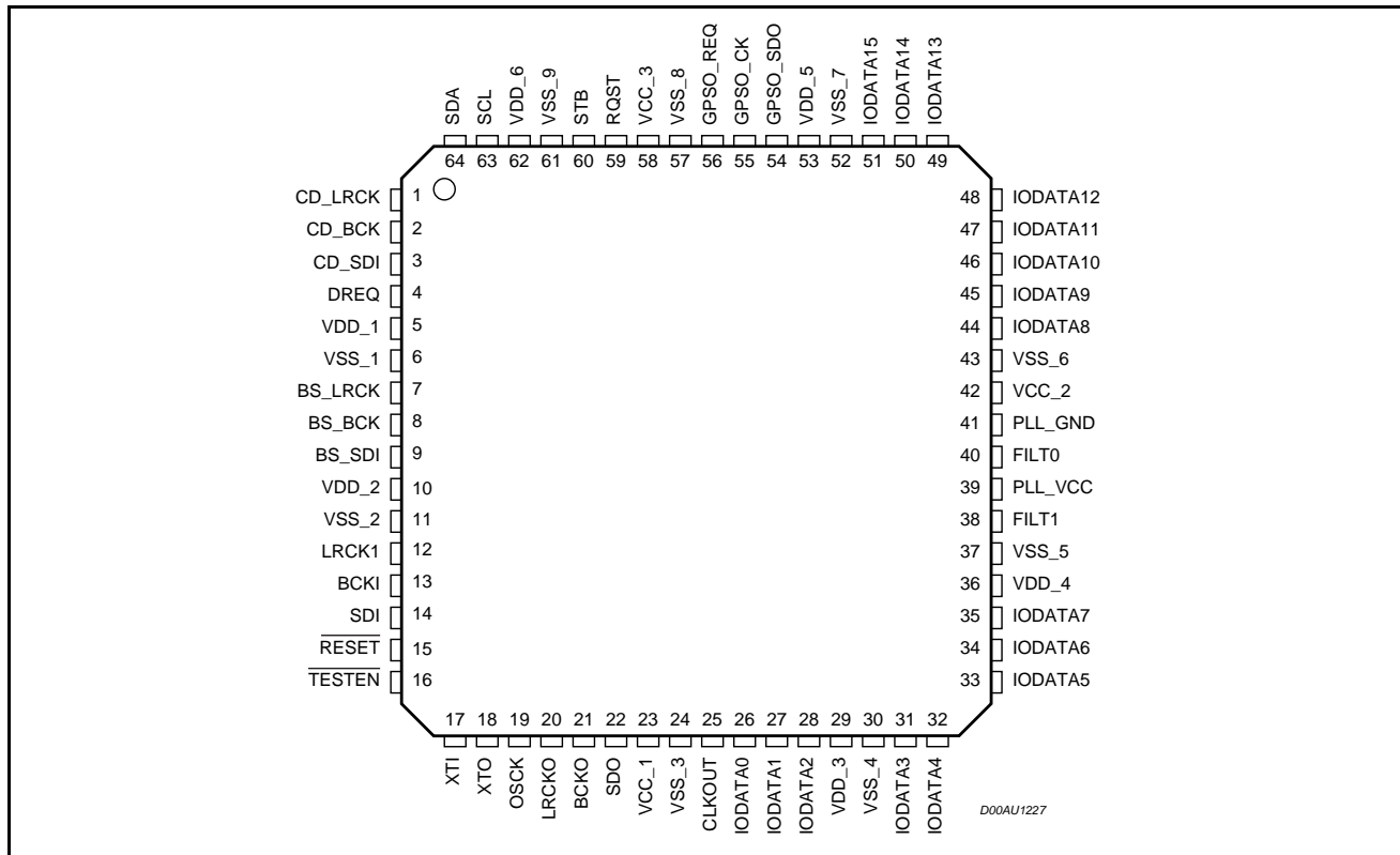
Figure 5. PIN CONNECTION
