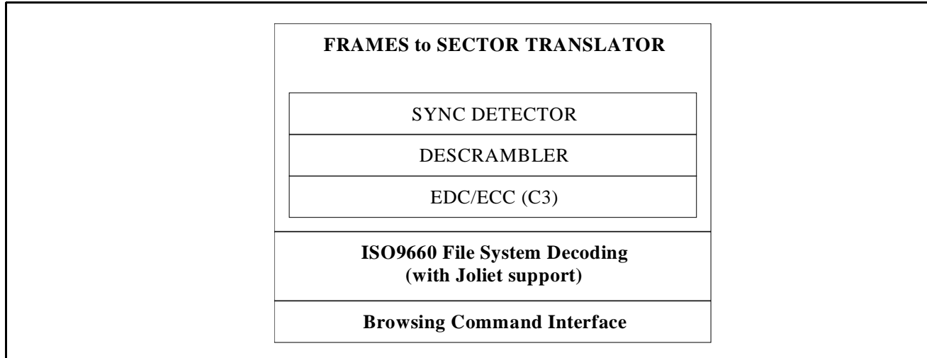
Figure 4. Layers performed by embedded DSP firmware
