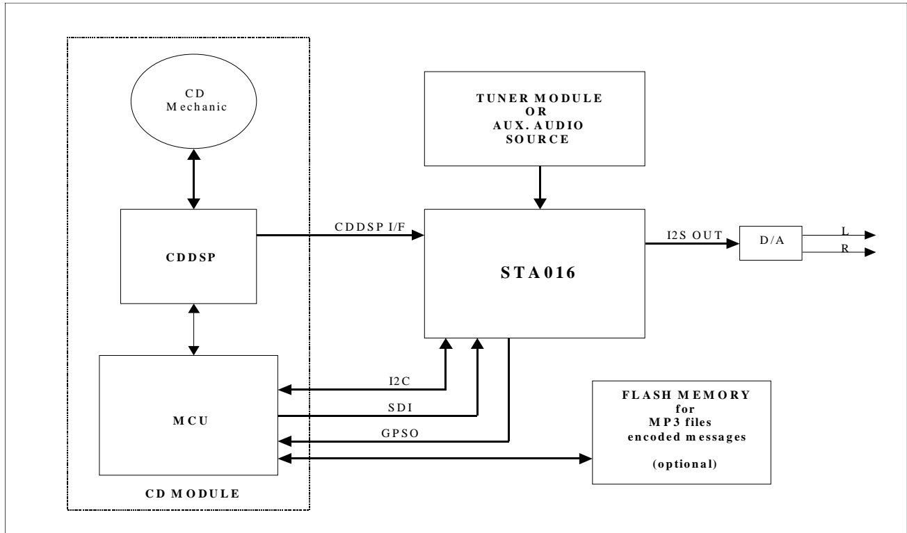
Figure 2. Typical CD-Player application
