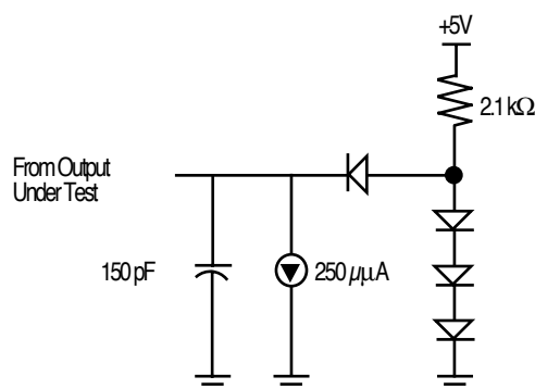
FIGURE 7. STANDARD TEST LOAD
