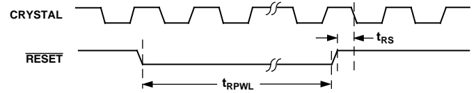
Figure 27. Reset Timing
