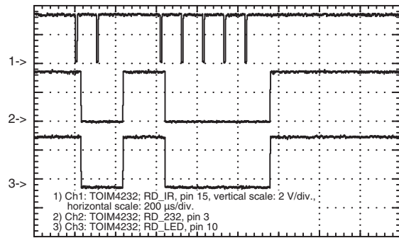
Fig. 8 - Data reception with the setting 9.6 kbit/s. Same as in figure 7, extended pulse duration
