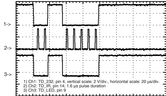
Fig. 6 - Data transmission with the setting 115.2 kbit/s, 1.627 µs pulse duration. By definition, the pulse duration of 1.627 µs is identical to the 3/16-bit pulse width.
