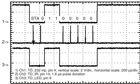
Fig. 4 - Data transmission with 9.6 kbit/s, 1.627 µs pulse duration
