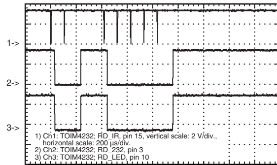
Fig. 7 - Data reception with the setting 9.6 kbit/s. Short RXD pulse
