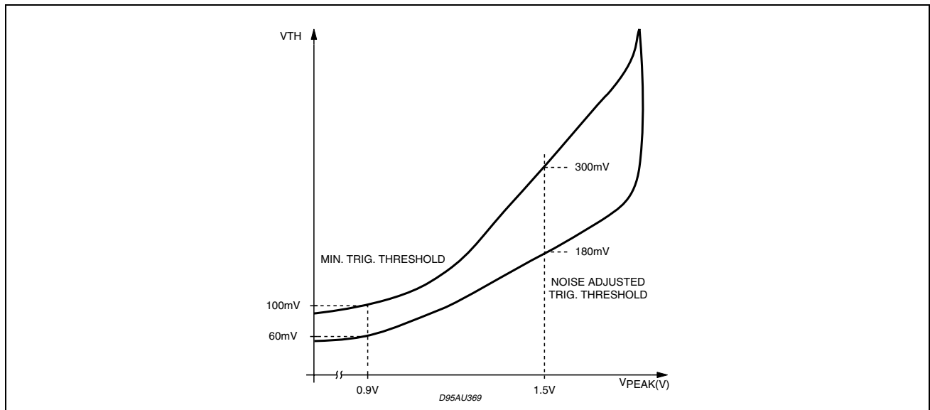
Figure 8. Trigger Threshold vs. V PEAK
