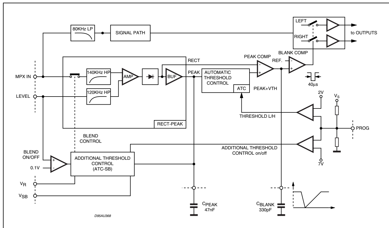
Figure 7. Block Diagram of the Noise Blanker
