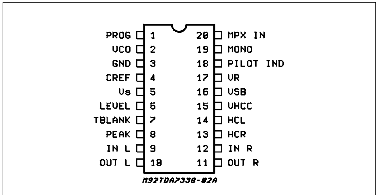
Figure 2. Pinout Diagram
