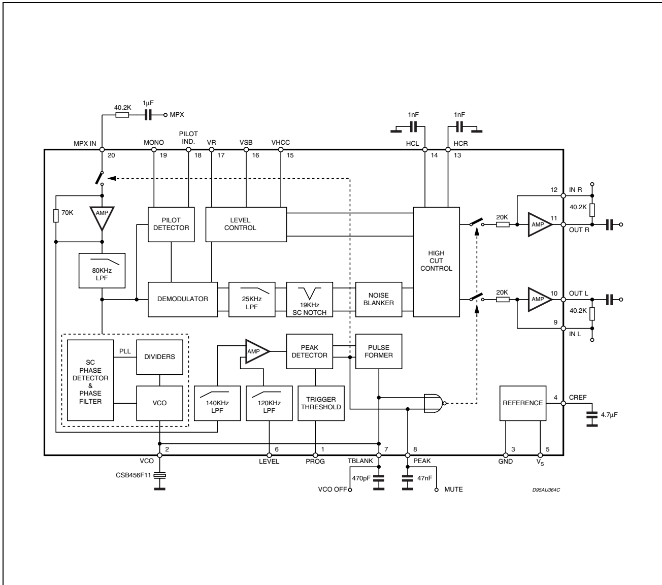
Figure 3. Block Diagram and Test Circuit
