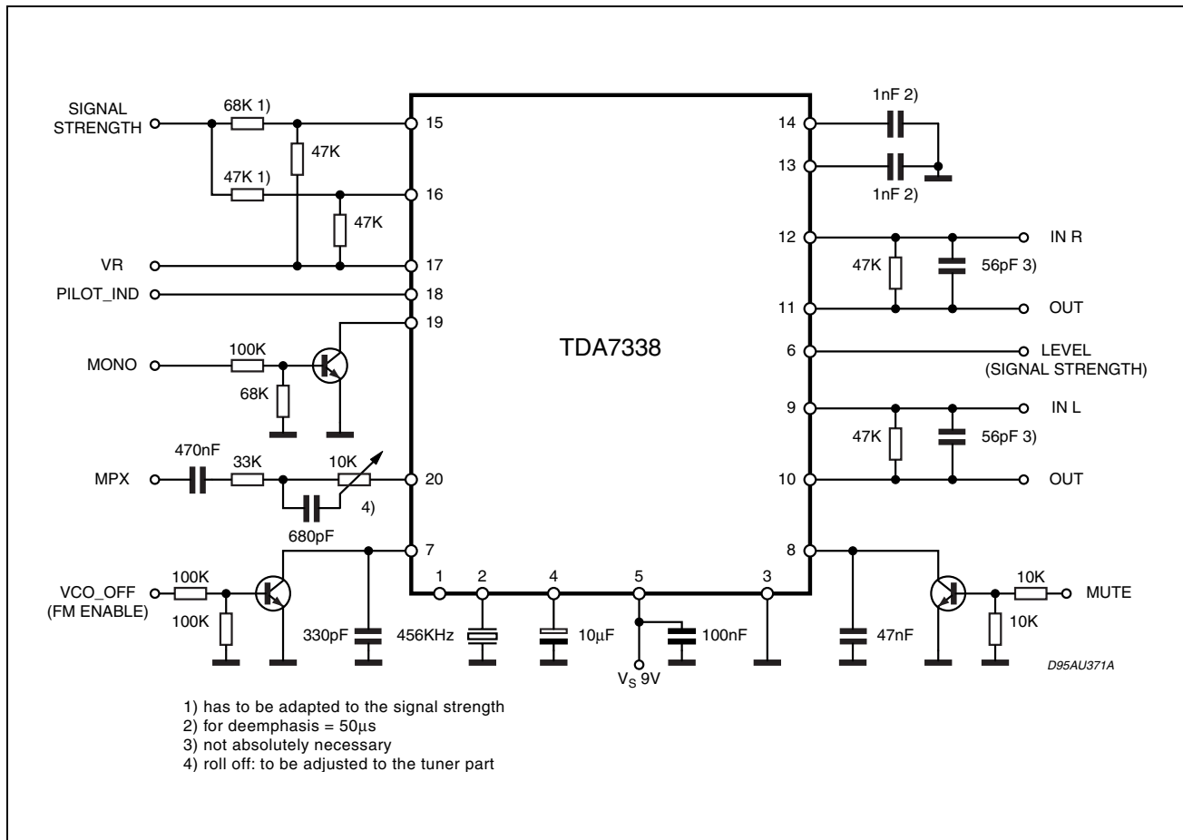
Figure 10. Application Diagram
