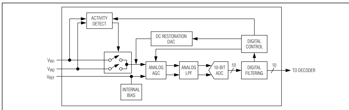
Figure 1. Analog Front-End
