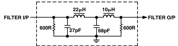
Figure 101. Output Filter for 4× Oversampling Mode
