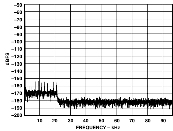
TPC 11. Wideband FFT Plot (16k Points) 44.1 kHz:192 kHz, -60 dBFS 1 kHz Tone
