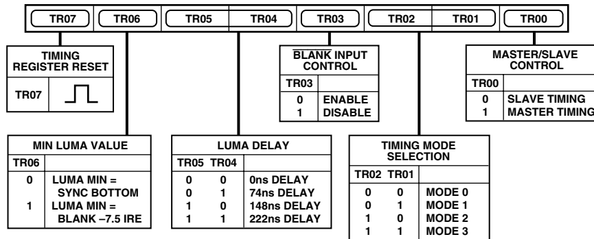
Figure 52. Timing Register 0
