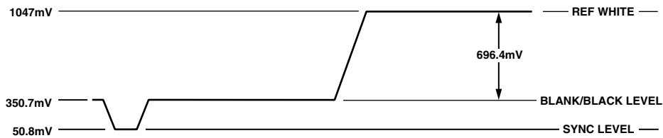
Figure 83. PAL Luma Video Levels
