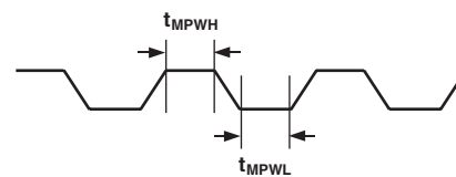
Figure 3. MCLK_IN Timing
