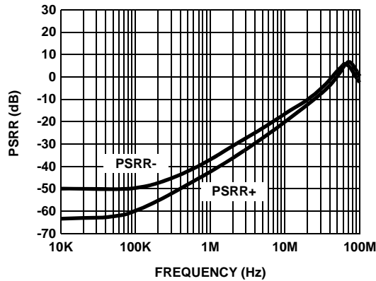
FIGURE 48. POWER SUPPLY REJECTION vs FREQUENCY
