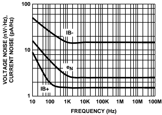
FIGURE 49. VOLTAGE AND CURRENT NOISE vs FREQUENCY
