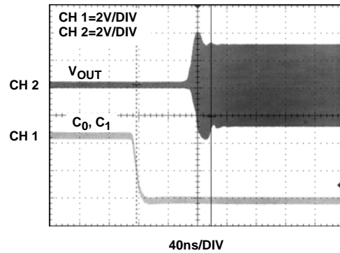
FIGURE 40. ENABLE TIME
