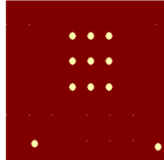
INTERNAL GROUND PLANE (16 Ld QFN)
