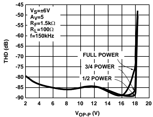
FIGURE 22. DIFFERENTIAL TOTAL HARMONIC DISTORTION vs DIFFERENTIAL OUTPUT VOLTAGE
