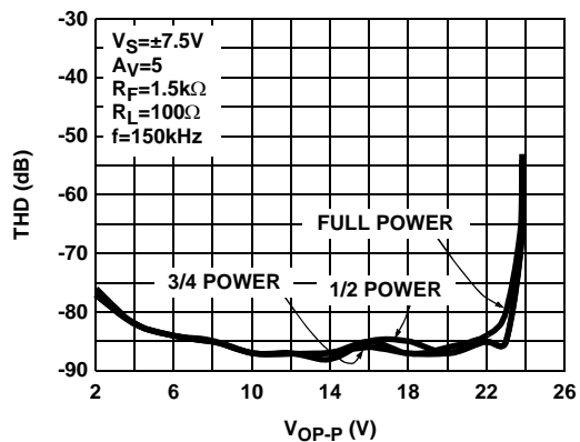
FIGURE 24. DIFFERENTIAL TOTAL HARMONIC DISTORTION vs DIFFERENTIAL OUTPUT VOLTAGE
