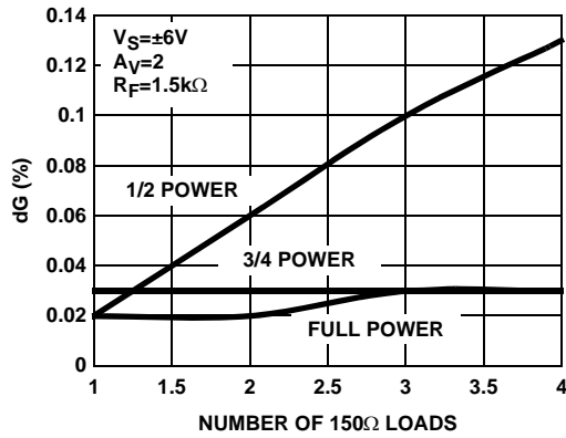
FIGURE 37. DIFFERENTIAL GAIN
