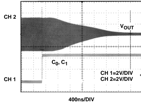
FIGURE 38. DISABLE TIME
