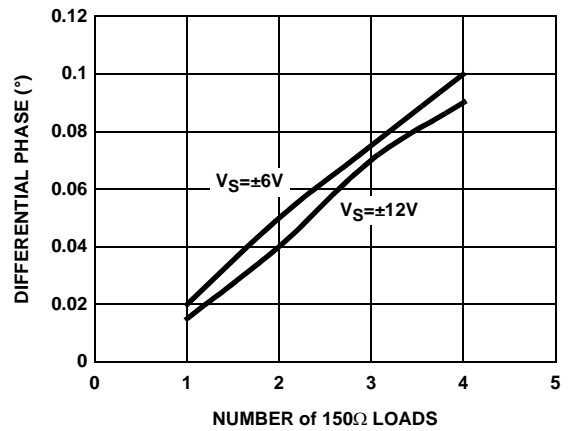
FIGURE 18. DIFFERENTIAL PHASE
