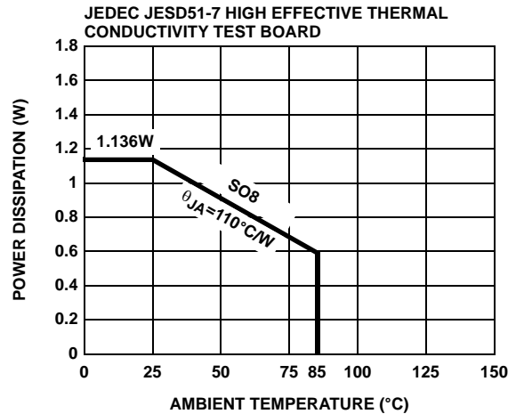
FIGURE 26. PACKAGE POWER DISSIPATION vs AMBIENT TEMPERATURE
