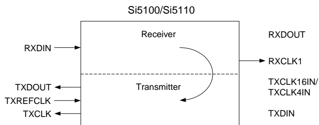
Figure 5. Line Loopback
