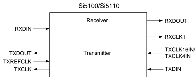
Figure 6. Full Duplex
