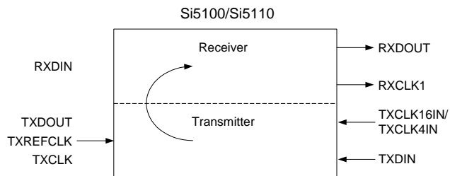
Figure 7. Diagnostic Loopback
