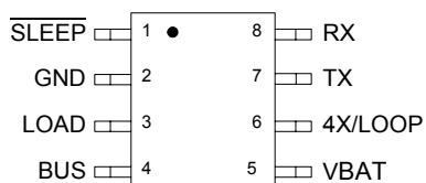
Figure 3. 33990 Pin Connections
