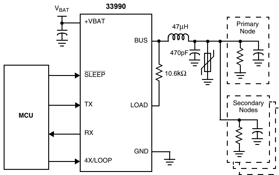
Figure 14. Typical Application
