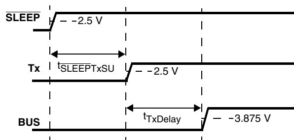
Figure 8. SLEEP to Tx Delay Times
