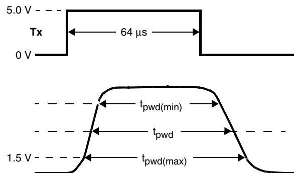
Figure 7. Pulse Width Distortion
