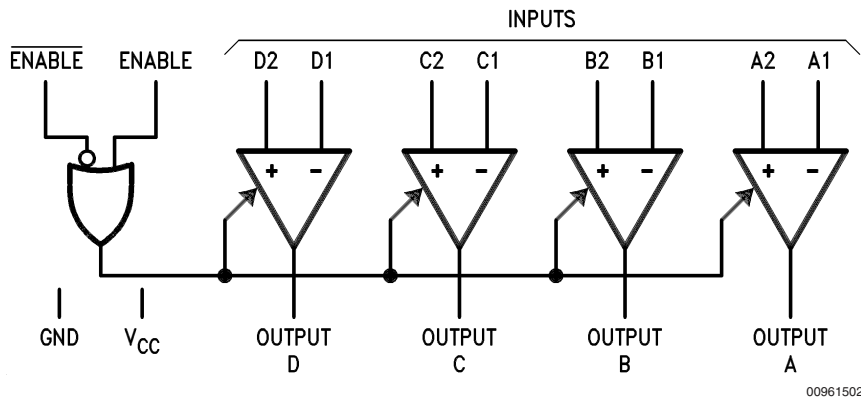
FIGURE 1. Logic Symbol
