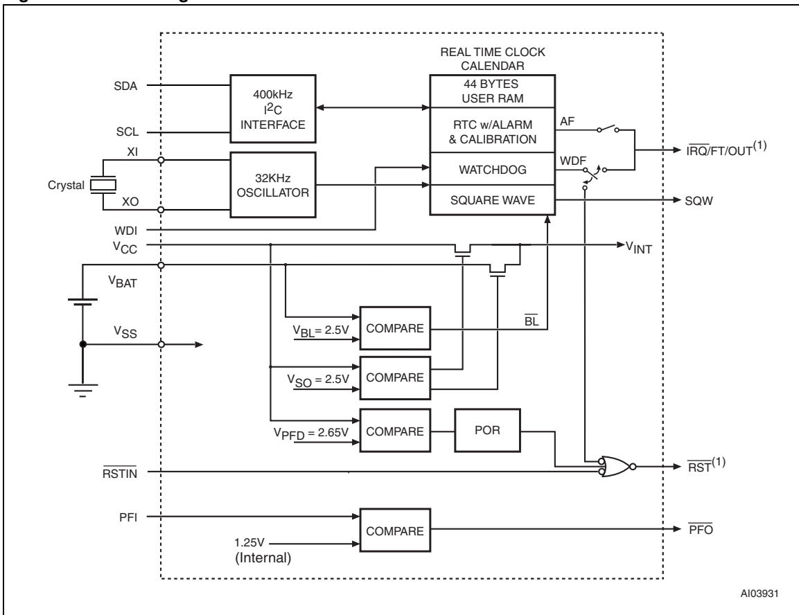
Figure 3. Block diagram
