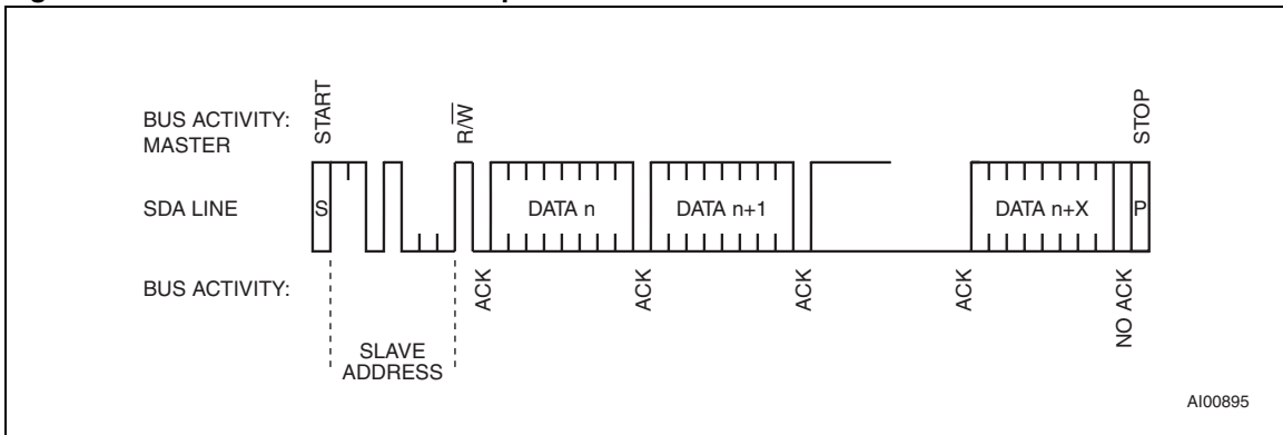
Figure 10. Alternate READ mode sequence
