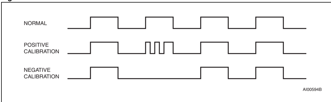
Figure 13. Clock calibration
