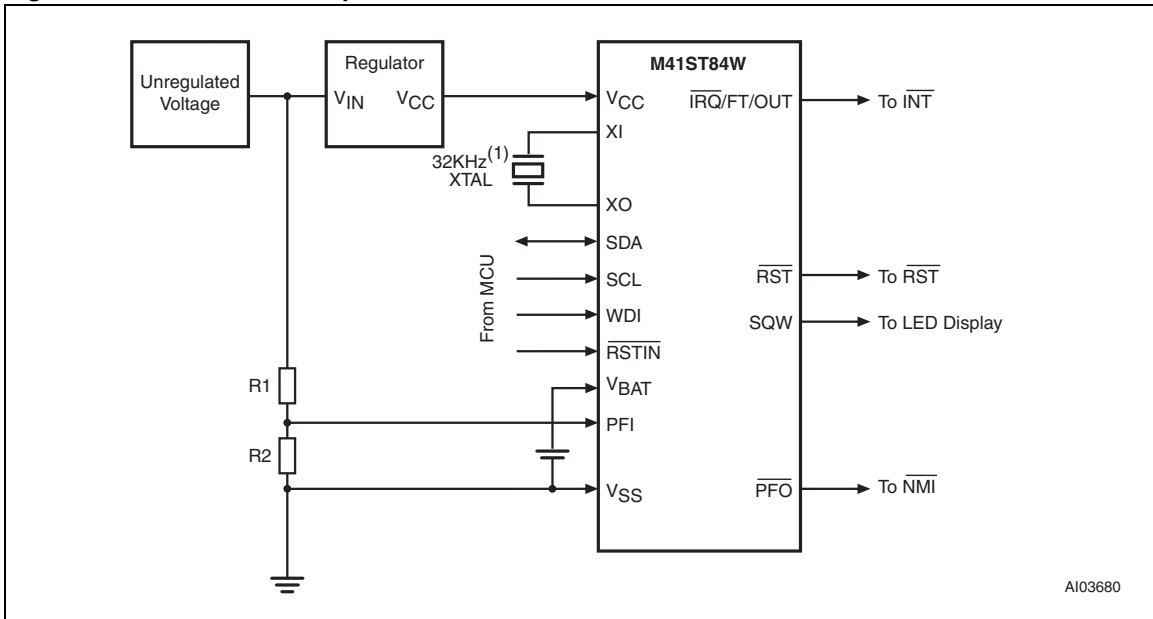
Figure 4. Hardware hookup
