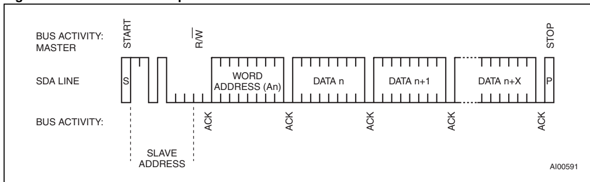
Figure 11. WRITE mode sequence
