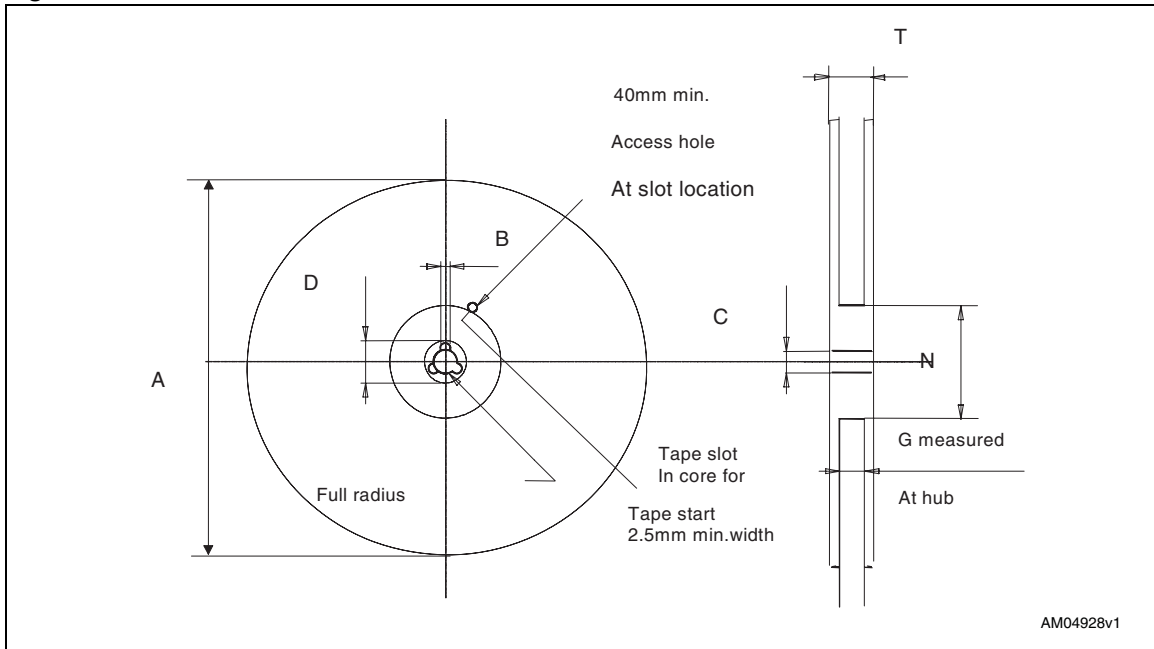
Figure 21. Reel schematic
