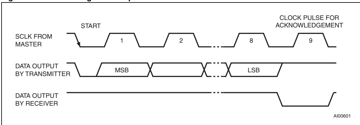
Figure 6. Acknowledgement sequence
