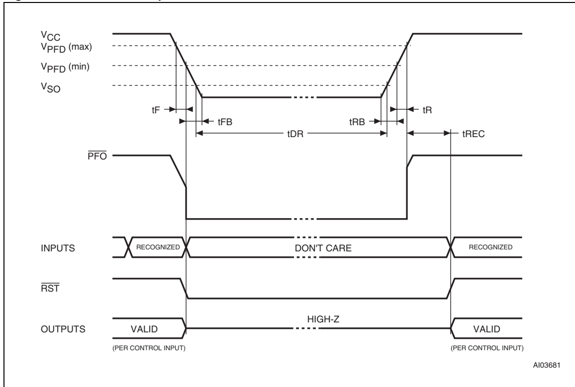
Figure 18. Power down/up mode AC waveforms
