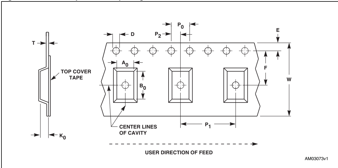
Figure 20. Carrier tape for SO16 package
