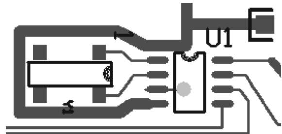
FIGURE 19. SUGGESTED LAYOUT FOR ISL12022 AND CRYSTAL
