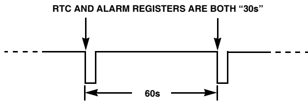
FIGURE 13. \overline{\text{IRQ}}/\text{F}_{\text{OUT}} WAVEFORM
