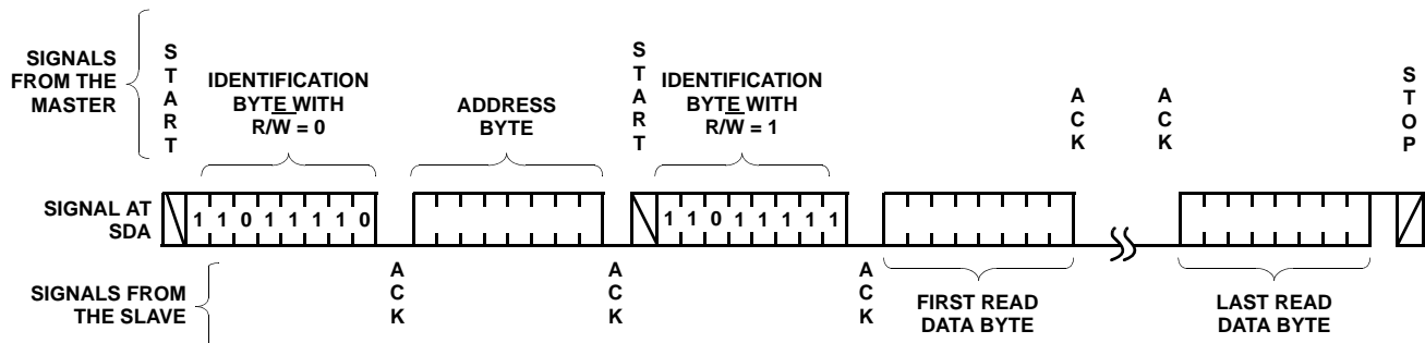
FIGURE 20. READ SEQUENCE (CSR SLAVE ADDRESS SHOWN)
