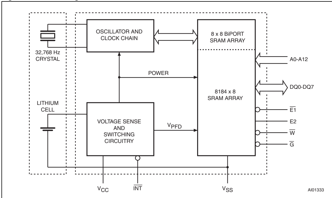
Figure 4. Block diagram
