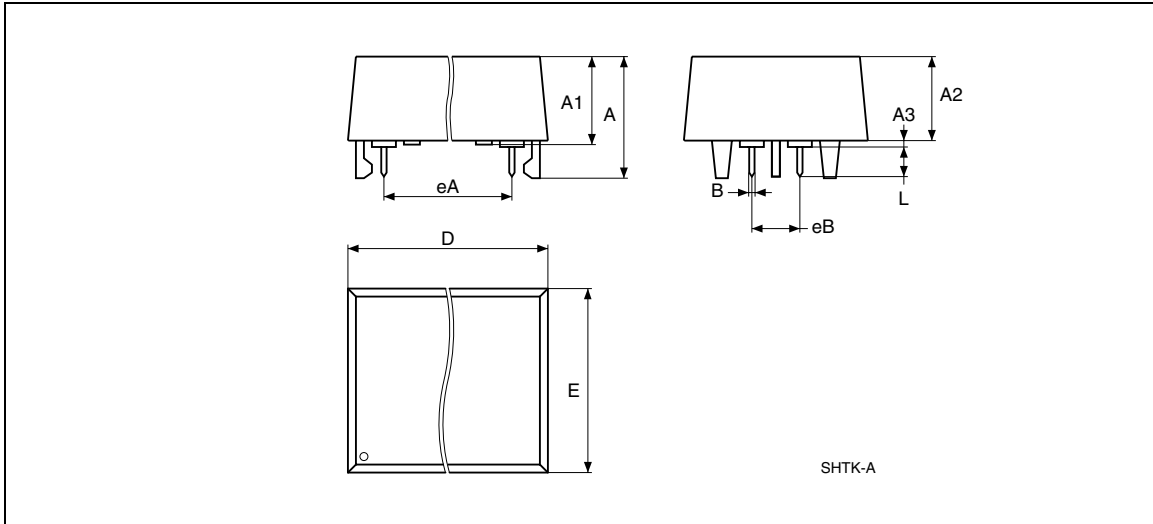
Figure 22. SH – 4-pin SNAPHAT® housing for 48 mAh battery &amp; crystal, package outline
