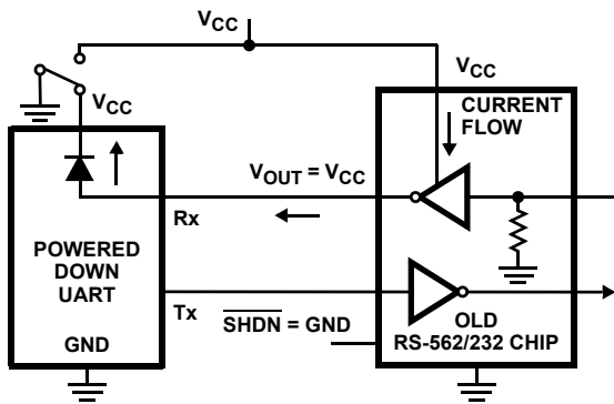
FIGURE 4. POWER DRAIN THROUGH POWERED DOWN PERIPHERAL
