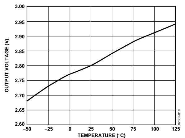
Figure 18. Driver Differential Output Voltage vs. Temperature ( R_{L\text{DIFF}} = 53.6 \Omega )
