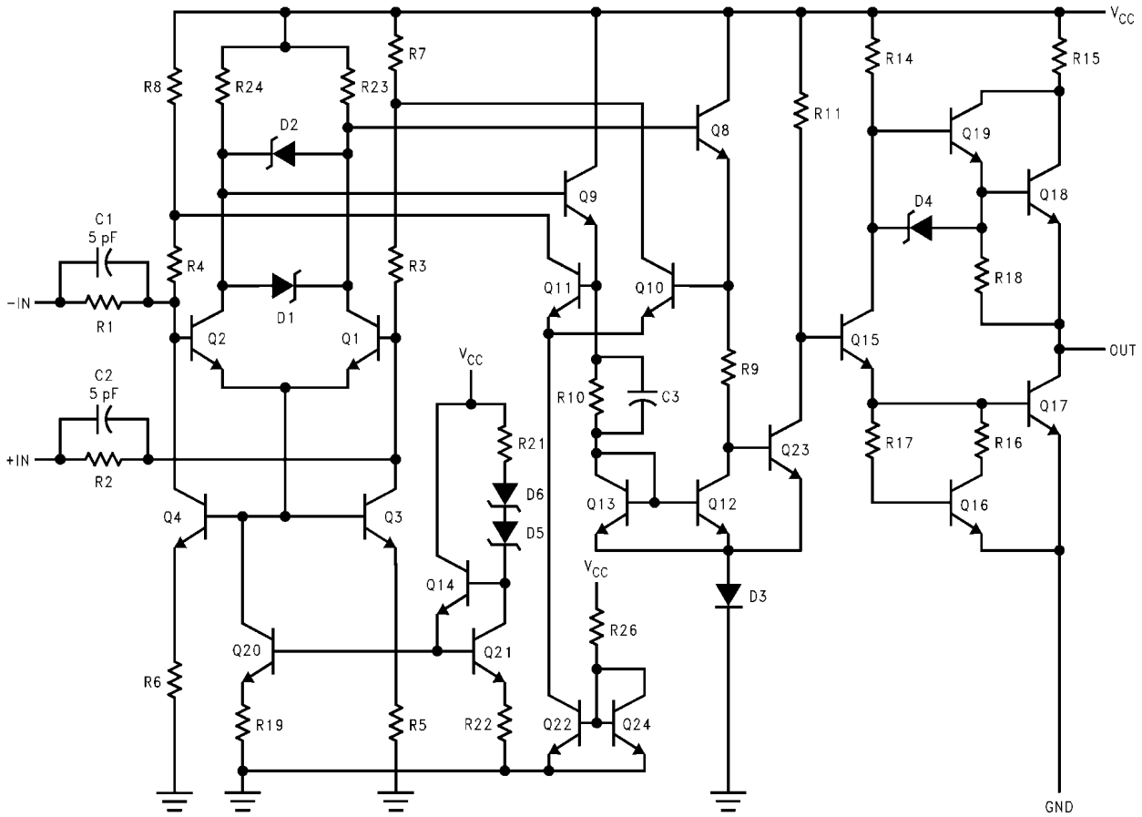
FIGURE 1. Equivalent Circuit
