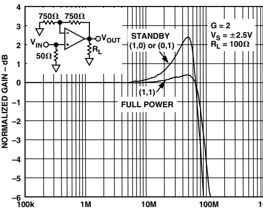
TPC 11. Small Signal Frequency Response
