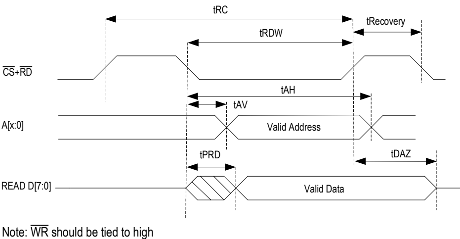
Figure-35 Non_multiplexed Intel Read Timing
