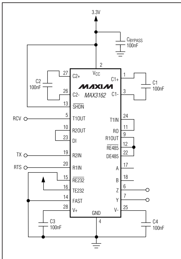
Figure 15. Protocol Translator
