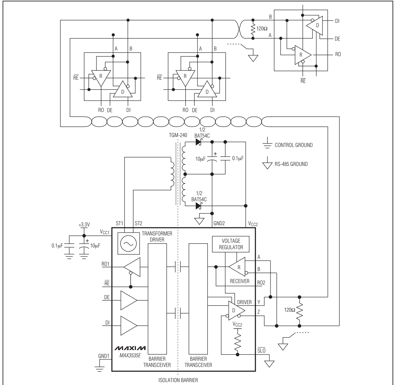
Figure 11. Typical Half-Duplex Multidrop RS-485 Network
