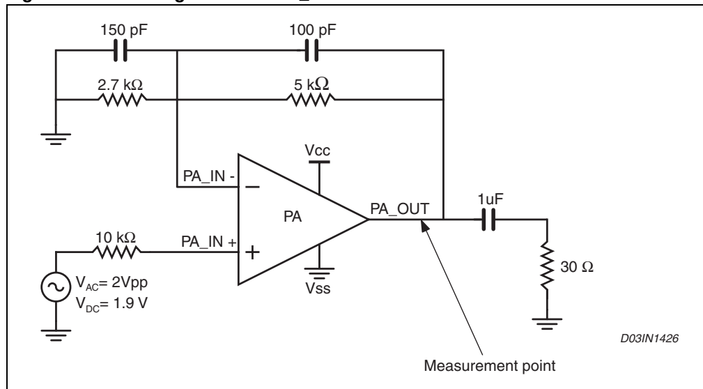
Figure 3. PLI configuration for PA_OUT distortions measurement
