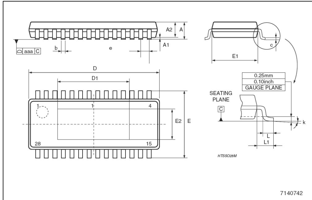
Figure 26. Package dimensions
