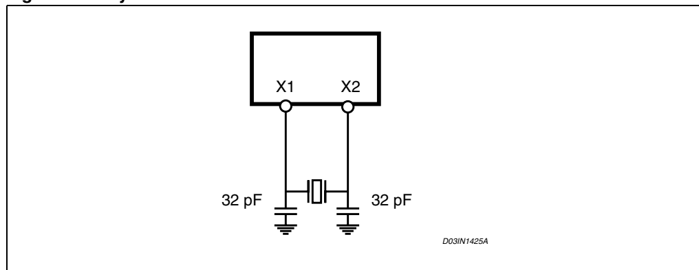
Figure 5. Crystal Resonator
