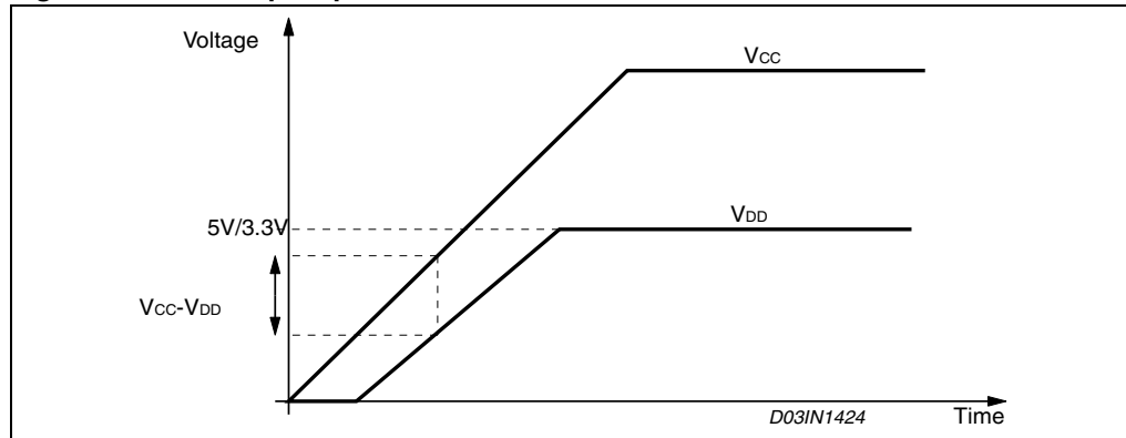
Figure 24. Power-up sequence
