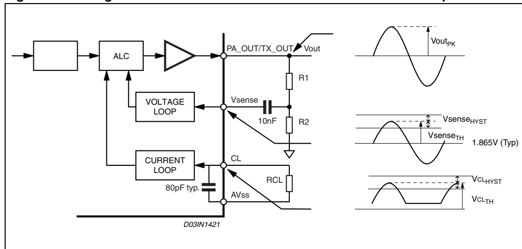
Figure 17. Voltage and current feedback external interconnection example
