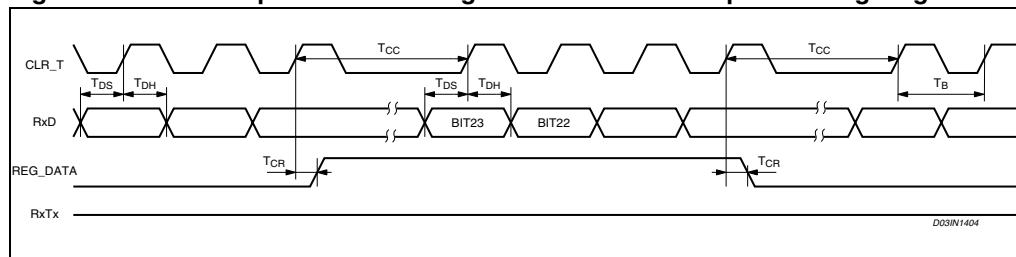
Figure 10. data reception - control register write - data reception timing diagram
