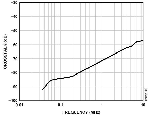
Figure 8. Crosstalk vs. Frequency, Typical ADSL/ADSL+ Application Circuit, V_{OUT} = 2 V p-p, R_L = 100 \Omega
