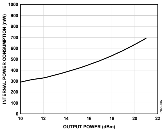
Figure 7. Internal Power Consumption vs. Output Power, Typical ADSL/ADSL+ Application Circuit, 100 \Omega Resistive Load Only
