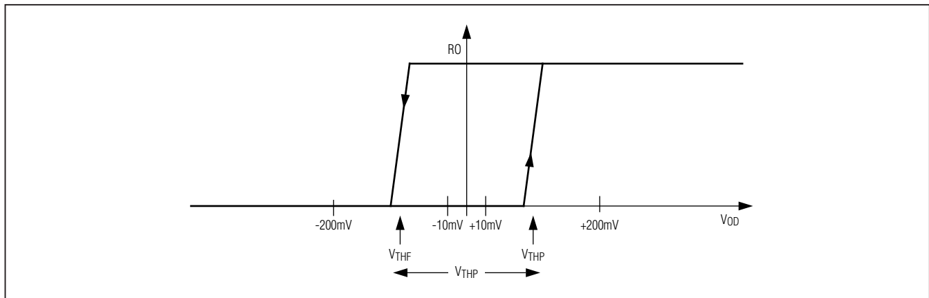
Figure 9. Symmetrical Hysteresis
