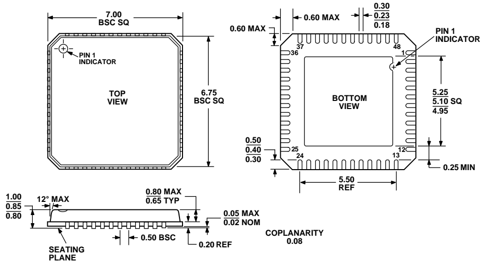
Figure 8. 48-Lead Frame Chip Scale Package [LFCS] (CP-48)
