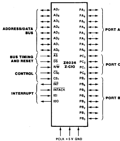
Figure 7-1. Z8036 (Z-CIO) Pin Functions
