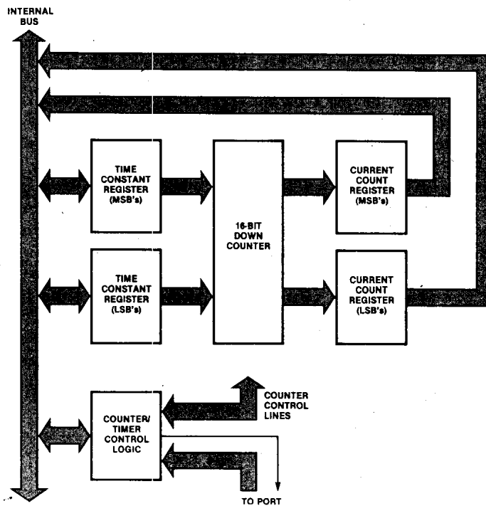
Figure 1-4. Counter/Timer Block Diagram
