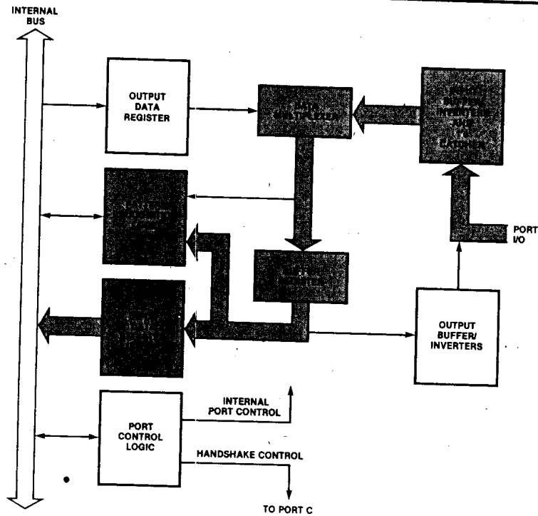
Figure 3-1. Input Port Data Path
