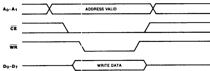
Figure 8-4. Z8536 (CIO) Write Cycle Timing
