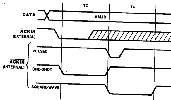
Figure 3-6. Pulsed Input Handshake Counter/Timer Duty Cycles
