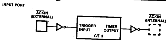
Figure 3-5. Pulsed Input Handshake Counter/Timer Insertion
