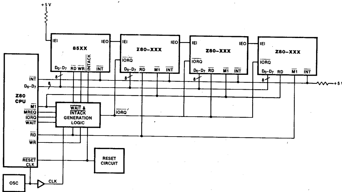
Figure 5-3. Non Z-Bus Interrupt Arbitration
