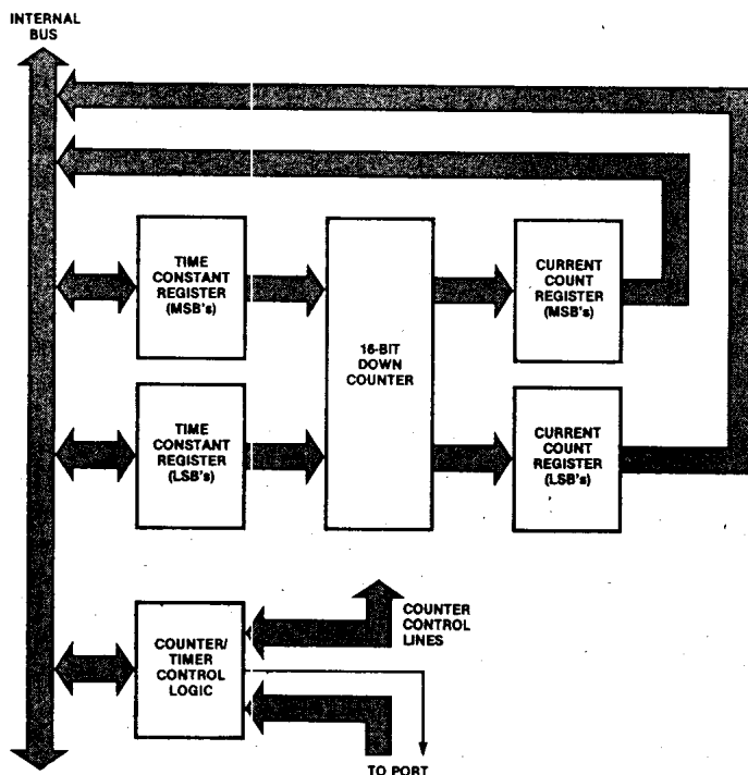
Figure 4-1. Counter/Timer Block Diagram
