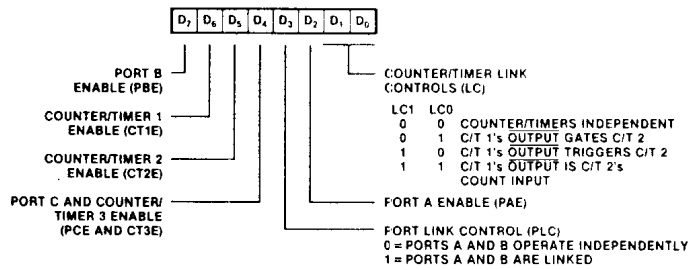
Figure B-1. Master Control Registers
