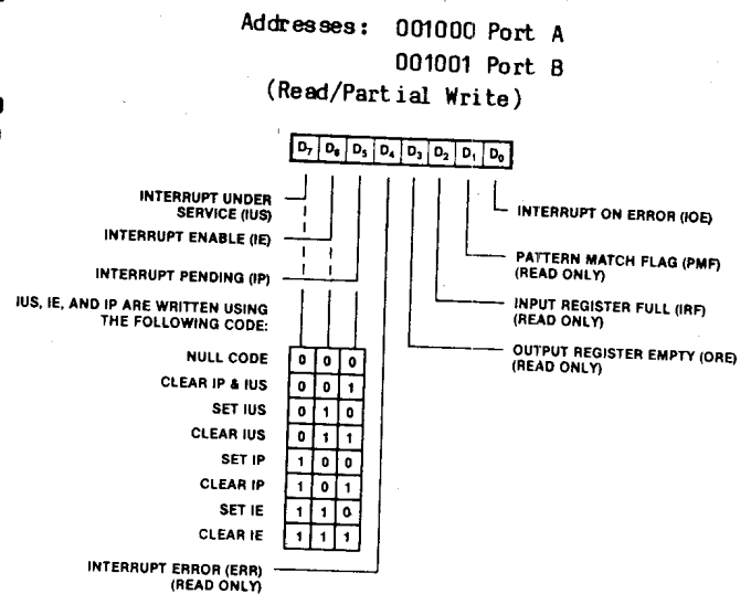
Figure 2-6. Port Command and Status Registers
