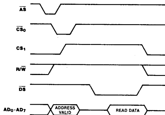
Figure 7-3. Z8036 (Z-CIO) Read Cycle Timing
