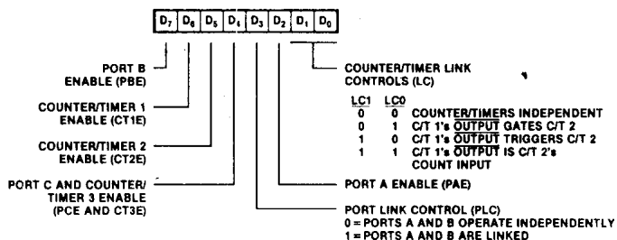
Figure 2-3. Master Configuration Control Register
