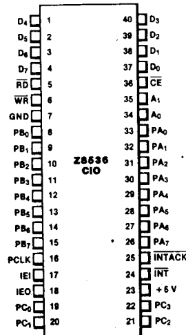
Figure 2. Pin Assignments
