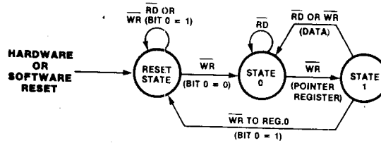
Figure 6-1. Z8536 State Machine Operation
