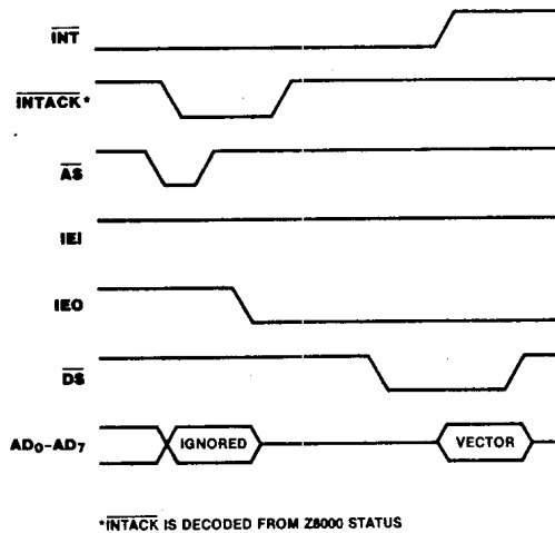
Figure 7-5. Z8036 (Z-CIO) Interrupt Acknowledge Timing
