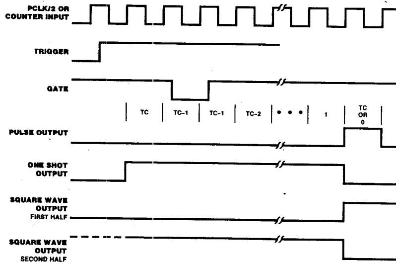
Figure 4-4. Counter/Timer Timing Diagram
