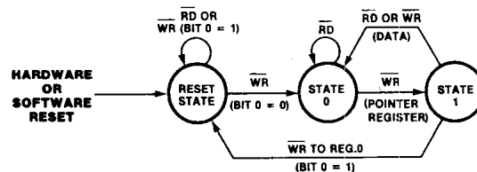
Figure 2-1. Z8536 State Machine Operation
