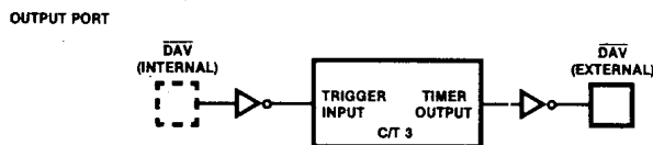
Figure 3-11. Pulsed Output Handshake Counter/Timer Insertion
