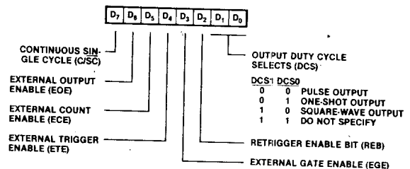
Figure 2-15. Counter/Timer Mode Specification Registers
