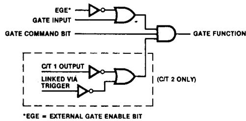
Figure 4-3. Gate AND-Function Diagram
