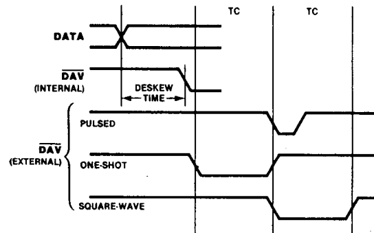
Figure 3-12. Pulsed Output Handshake Counter/Timer Duty Cycles
