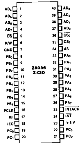
Figure 2. Pin Assignments
