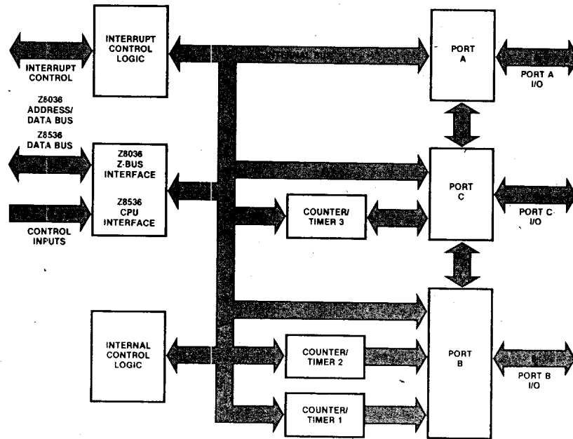
Figure 1-1. Z8036/Z8536 Z-C10/C10 Block Diagram
