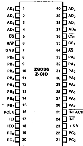
Figure 7-2. Z8036 (Z-CIO) Pin Assignments
