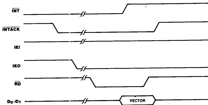
Figure 8-5. Z8536 (CIO) Interrupt Acknowledge Timing
