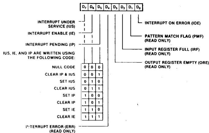
Figure B-2. Port Specification Registers
