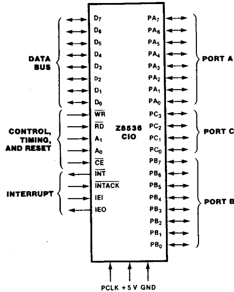
Figure 8-1. Z8536 (CIO) Pin Functions
