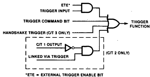
Figure 4-2. Trigger OR-Function Diagram
