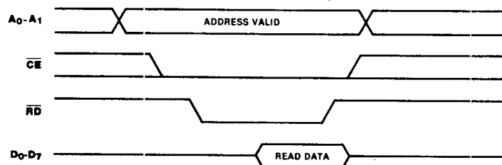
Figure 8-3. Z8536 (CIO) Read Cycle Timing
