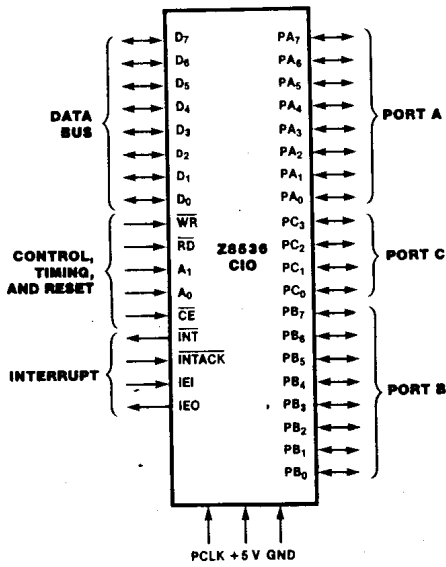
Figure 1. Pin Functions
