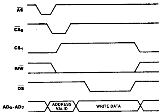
Figure 7-4. Z8036 (Z-CIO) Write Cycle Timing
