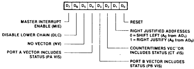
Figure B-1. Master Control Registers
