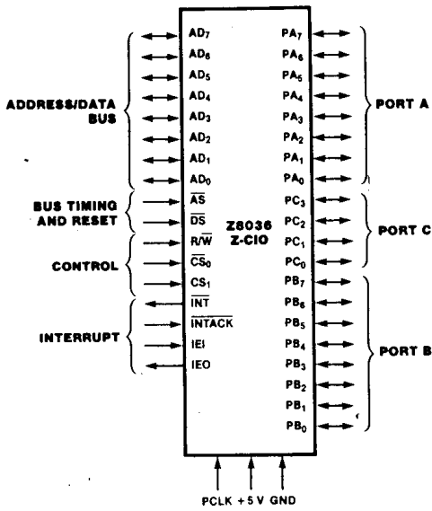
Figure 1. Pin Functions
