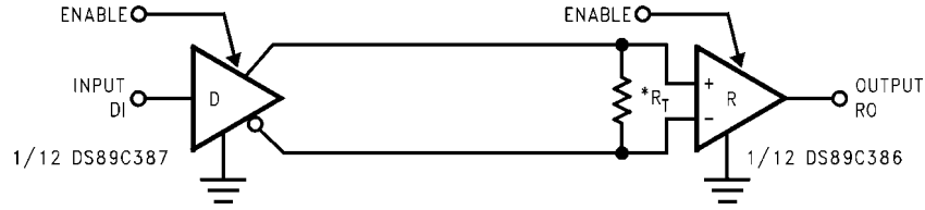
FIGURE 5. Two-Wire Balanced System, RS-422
