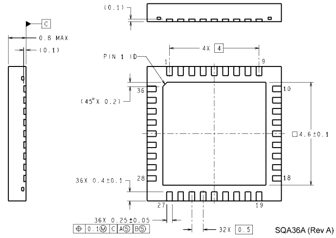
NS Package Number SQA36A
