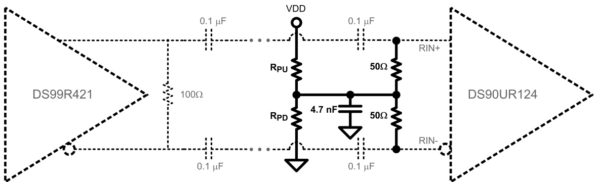
FIGURE 15. Receiver Termination Option 3
