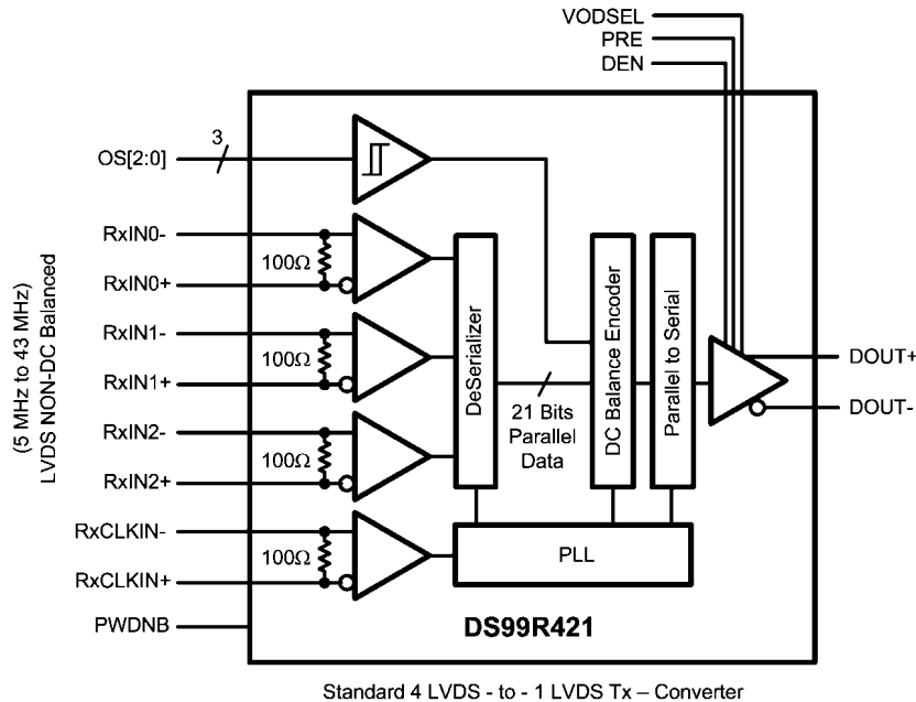
FIGURE 1. Block Diagram
