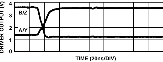
FIGURE 22. DRIVER AND RECEIVER WAVEFORMS, LOW TO HIGH (ISL83086E, ISL83088E)
