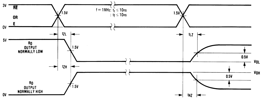
FIGURE 4. Receiver Enable/Disable Propagation Delay Timing
