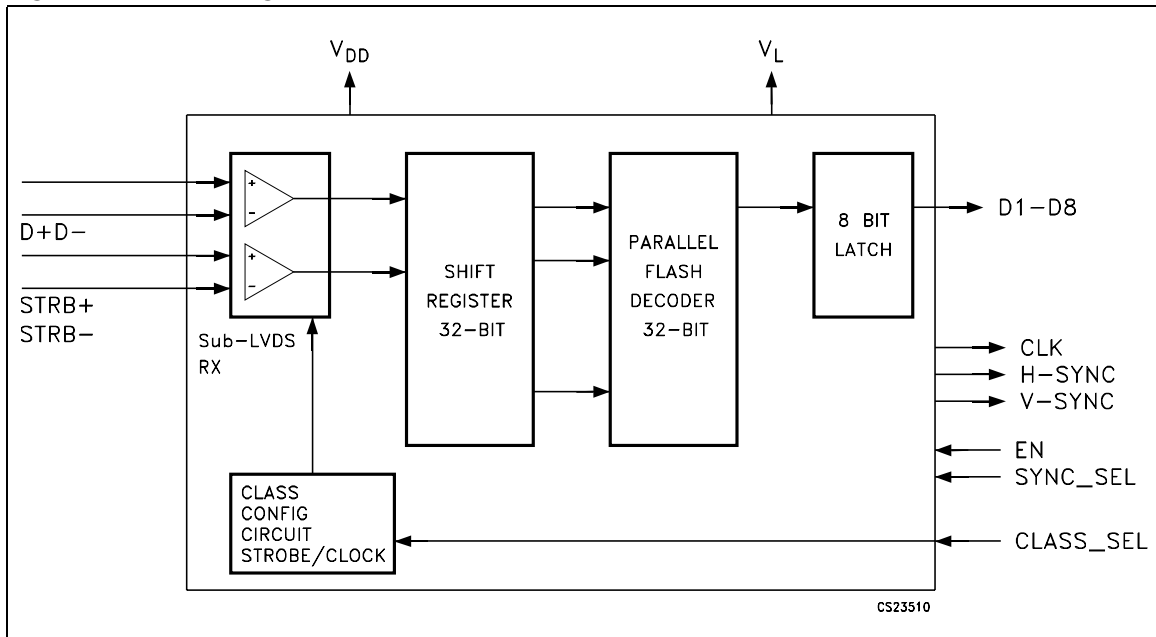
Figure 2. Block diagram
