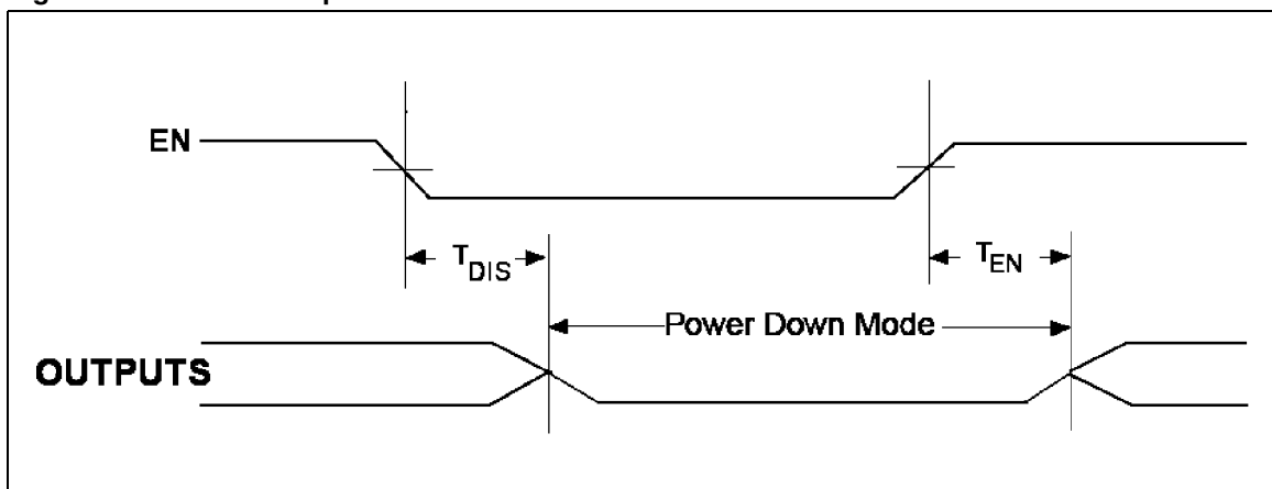
Figure 8. STSMIA832 power down mode
