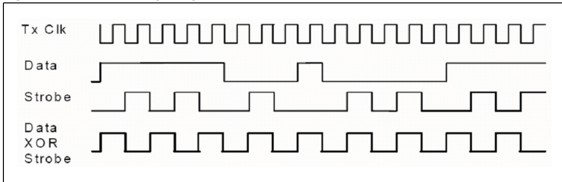
Figure 5. Data-strobe signaling
