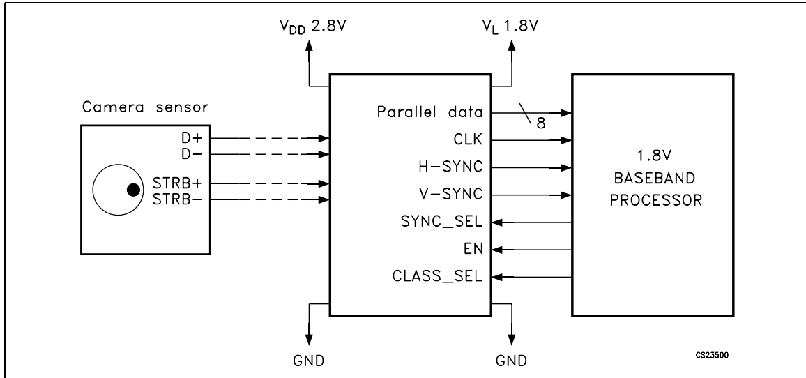
Figure 1. Simplified application block diagram
