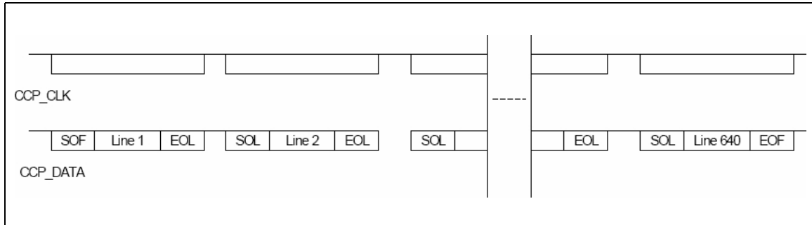
Figure 7. CCP2 synchronization codes
