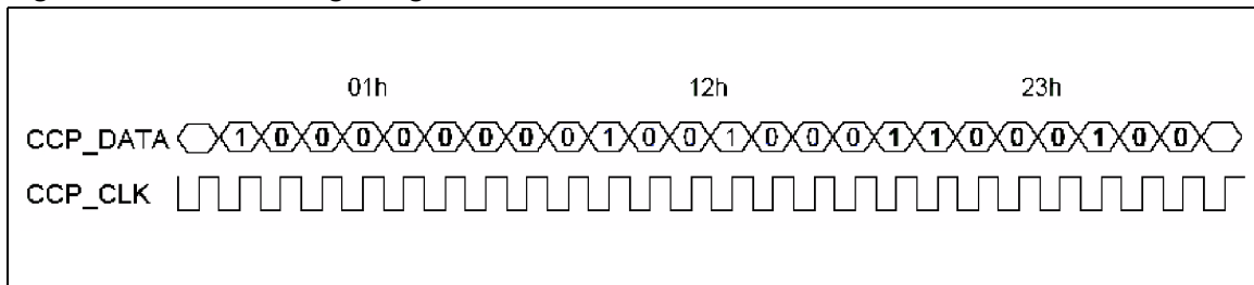
Figure 4. Data clock signaling
