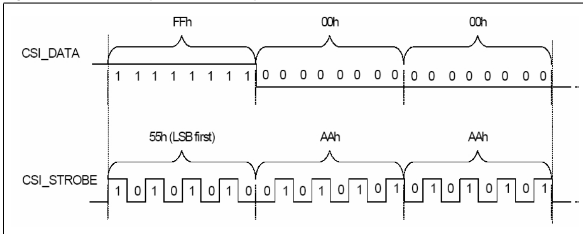
Figure 6. Data-strobe phase relationship
