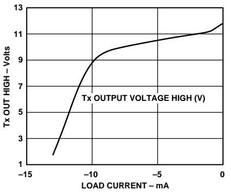
Figure 14. Transmitter Output Voltage High vs. Load Current
