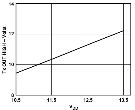
Figure 16. Transmitter Output Voltage High vs. V_{DD}
