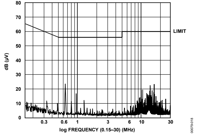
Figure 23. Conducted Emissions
