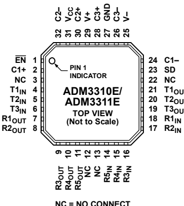
Figure 6. LFCSP_VQ Pin Configuration
