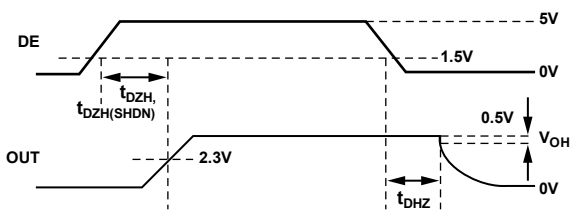
Figure 18. Driver Enable and Disable Times ( t_{DZH} , t_{DZH(SHDN)} , t_{DHZ} )
