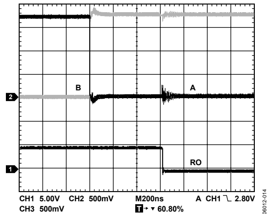
Figure 14. ADM483E Receiver t_{PLH} Driven by External RS-485 Device
